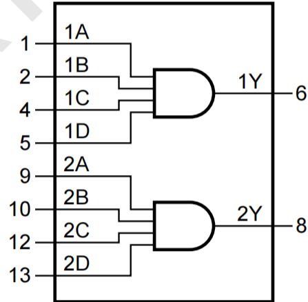
Figure 4. Functional diagram
