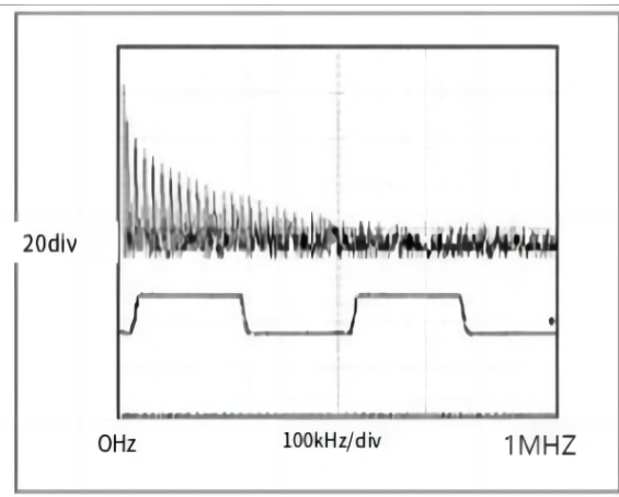
Figure 9: MAX490 driver when transmitting 20kHz signal
