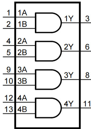
Figure 1. Logic symbol
