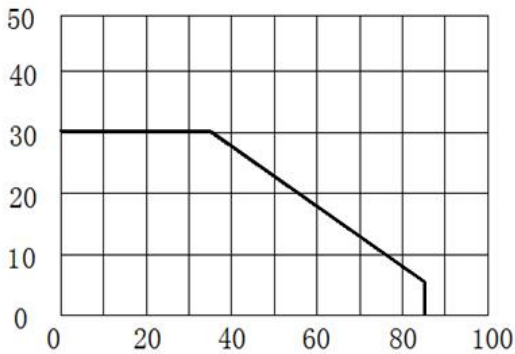
正向电流递减曲线图 Forward current decline curve
