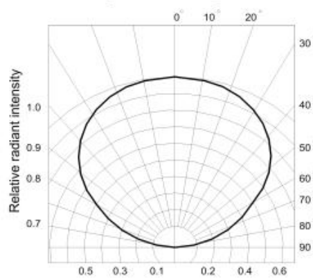
Fig.6 Radiation diagram
