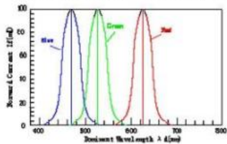
Typical Spectra (Ta=25°C) (Forward Current)
