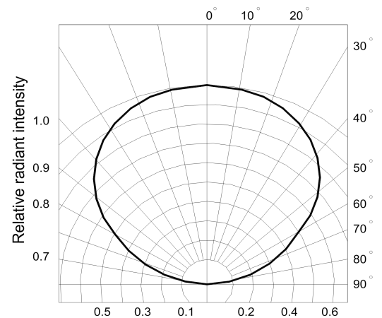
Fig.6 Radiation diagram
