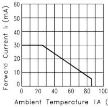
Fig.3 FORWARD CURRENT DERRATING CURVE
