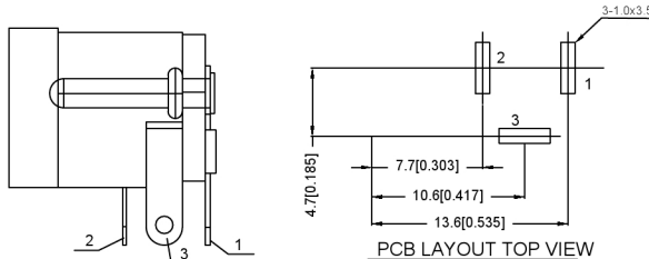
PCB LAYOUT TOP VIEW TOLERANCES: ±0.05
