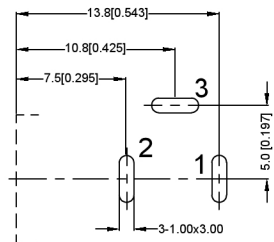
Pin Hole Layout Jack Bottom View
