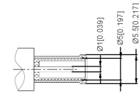
MATING PLUG Jack Insertion Depth: 9.0mm
