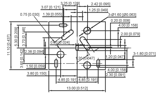
PCB LAYOUT TOP VIEW TOLERANCES:±0.05
