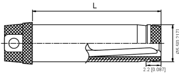
RECOMMENDED PLUG
