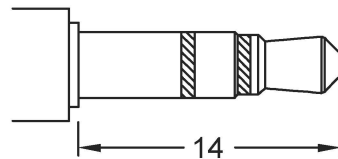
Ø3.5 MATING PLUG
