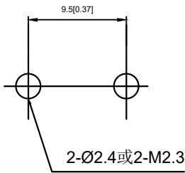
Solder and 110# Terminal
