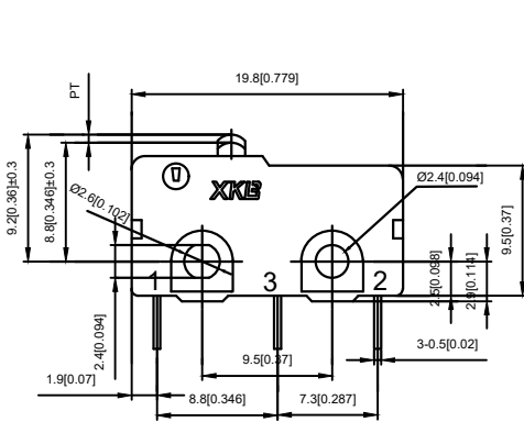
Solder and 110# Terminal
