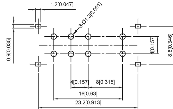
PCB LAYOUT
