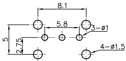
PCB board installation drawing (± 0.1)
