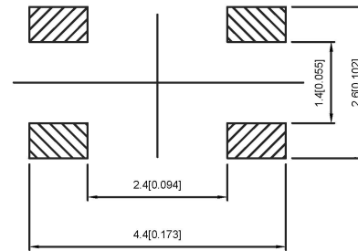
PCB.WELDING DRAWING
