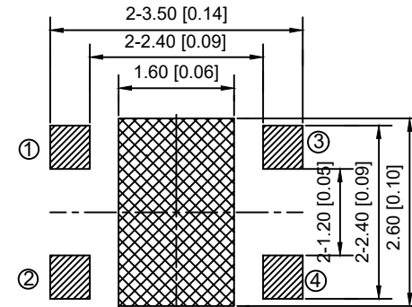
LAND PATTERN PLAN
