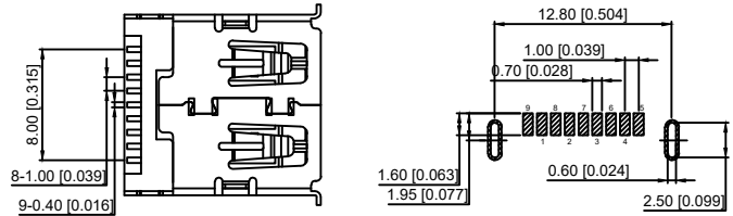
PCB
