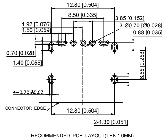
RECOMMENDED PCB LAYOUT (THK: 1.0MM)
