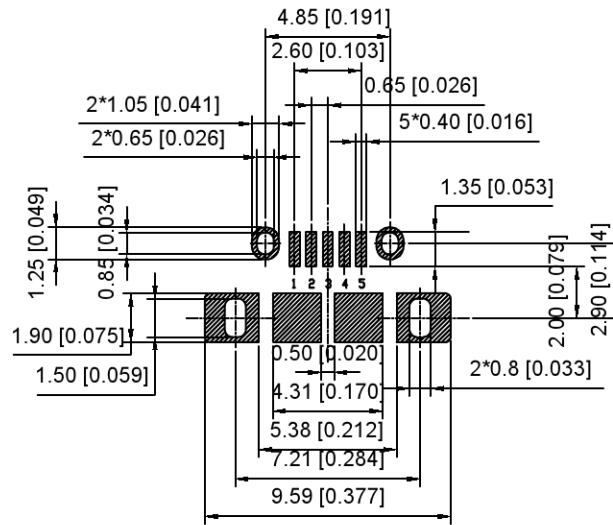
RECOMMENDED PCB LAYOUT(TOP VIEW) GENERAL TOLERANCES:±0.05
