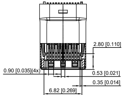
SECT B-B
