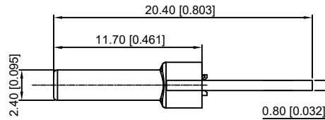
SECT B-B
