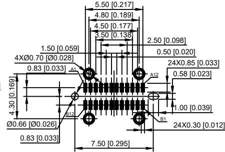
XKB RECOMMENDED P.C.B LAYOUT (T:1.00mm) TOLERANCE UNSPECIFIED ±0.05mm
