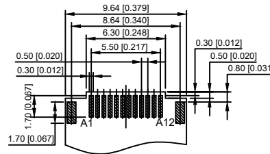
RECOMMENDED PCB LAYOUT(TOP VIEW) THICKNESS 0.80±0.05MM.DEFAULT TOLERANCE±0.05
