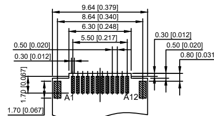
RECOMMENDED PCB LAYOUT(TOP VIEW) THICKNESS 0.80±0.05MM;DEFAULT TOLERANCE:±0.05
