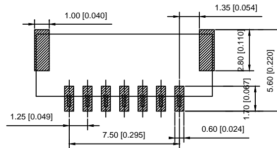
SUGGESD PCB LAYOUT (COMPONENT SIDE)
