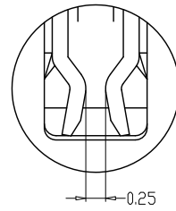
DETAIL "X"
