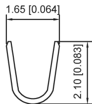
SECTION:A-A SCALE:1:1
