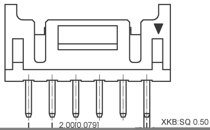
05P~13P Shape(Scale1:1)
