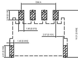
Mating PCB detail
