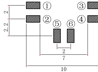
PCB LAYOT
