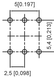
P.C.B LAYOUT BOTTOM VIEW
