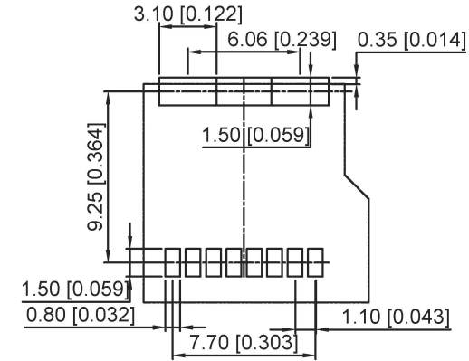
RECOMMENED P.C.B LAYOUT(TOP VIEW) GENERAL TOLERANCE ±0.05
