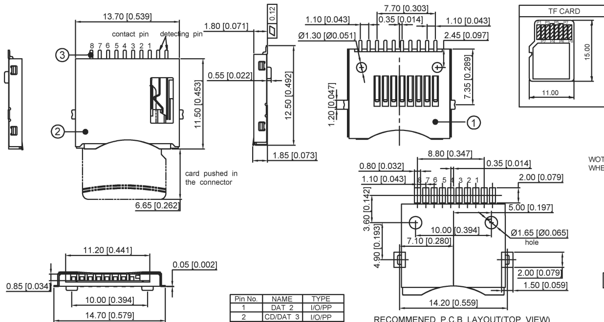
RECOMMEN P.C.B LAYOUT(TOP VIEW) GENERAL TOLERANCE ±0.05
