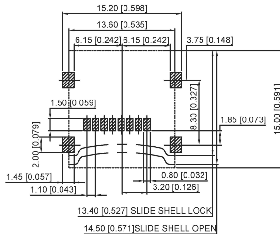
14.50 [0.571] SLIDE SHELL OPEN
