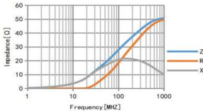
产品特性曲线图：Product Characteristic Curve
