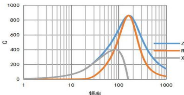
产品特性曲线图: Product Characteristic Curve
