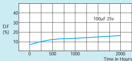
Dissipation Factor Change
