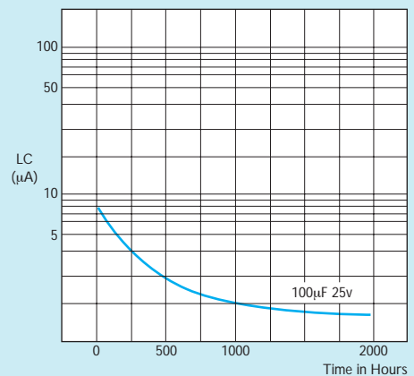
Leakage Current Change
