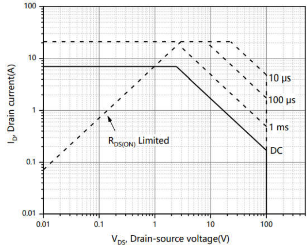
Figure 10. Safe operation area T_C=25\text{ °C}
