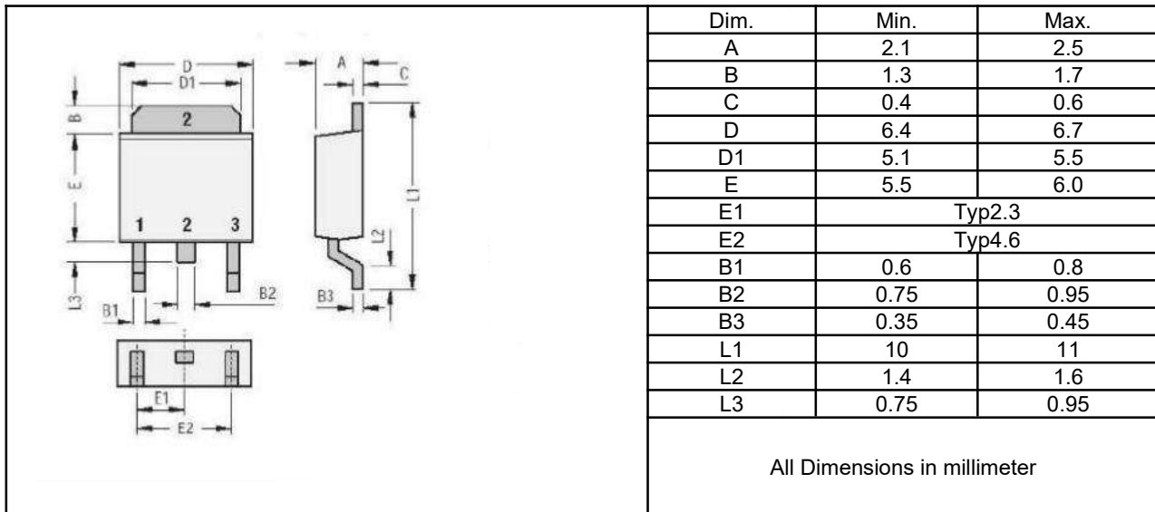
TO-252
