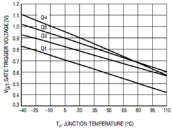
Figure 8. Typical Gate Trigger Voltage versus Junction Temperature
