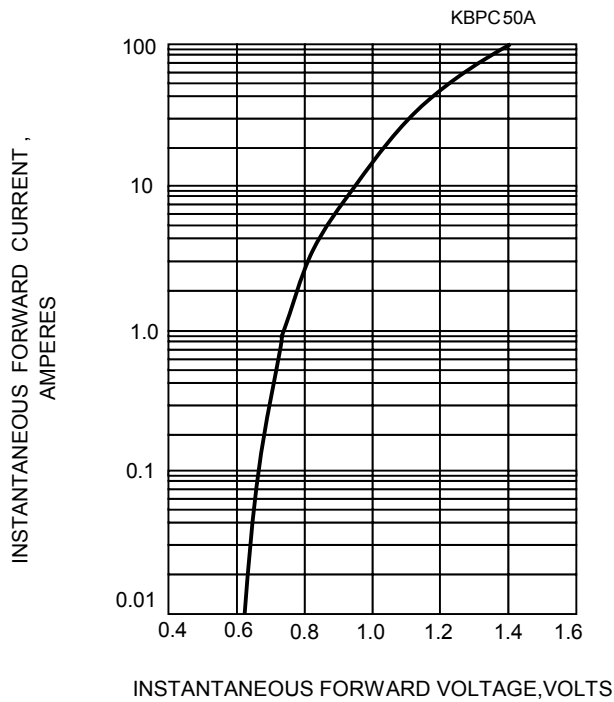
FIG.3-TYPICAL FORWARD CHARACTERISTICS
