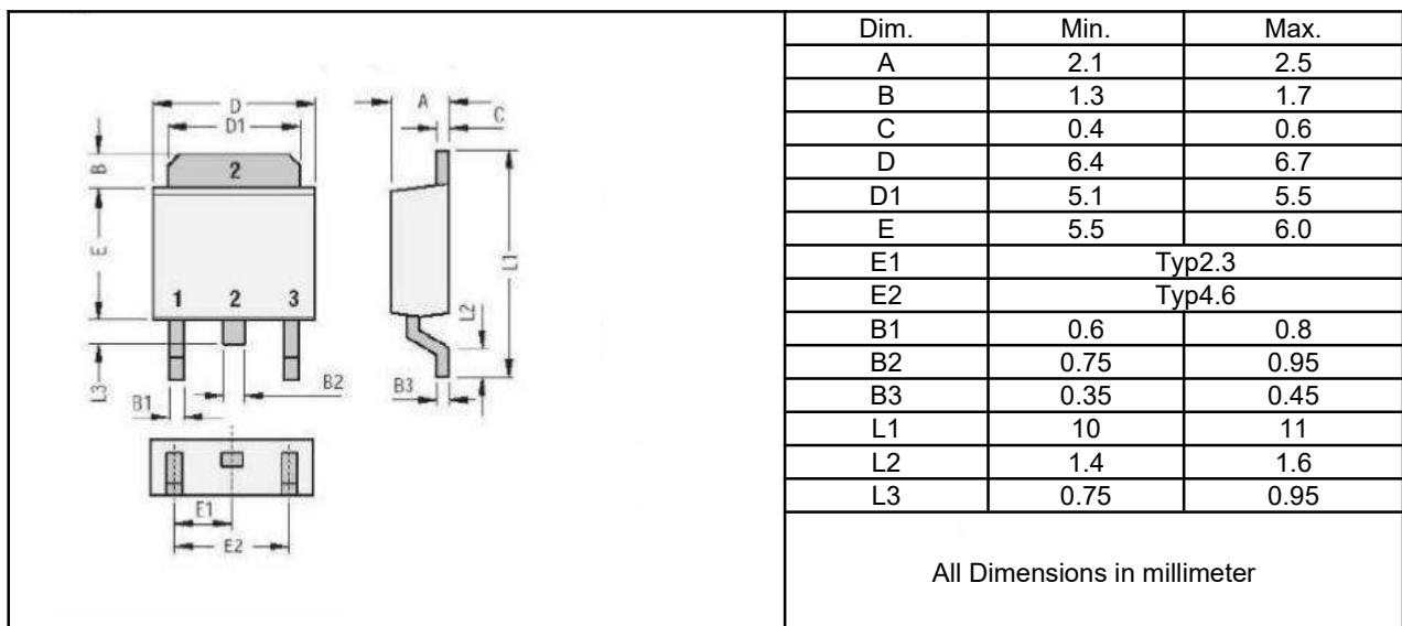
TO-252
