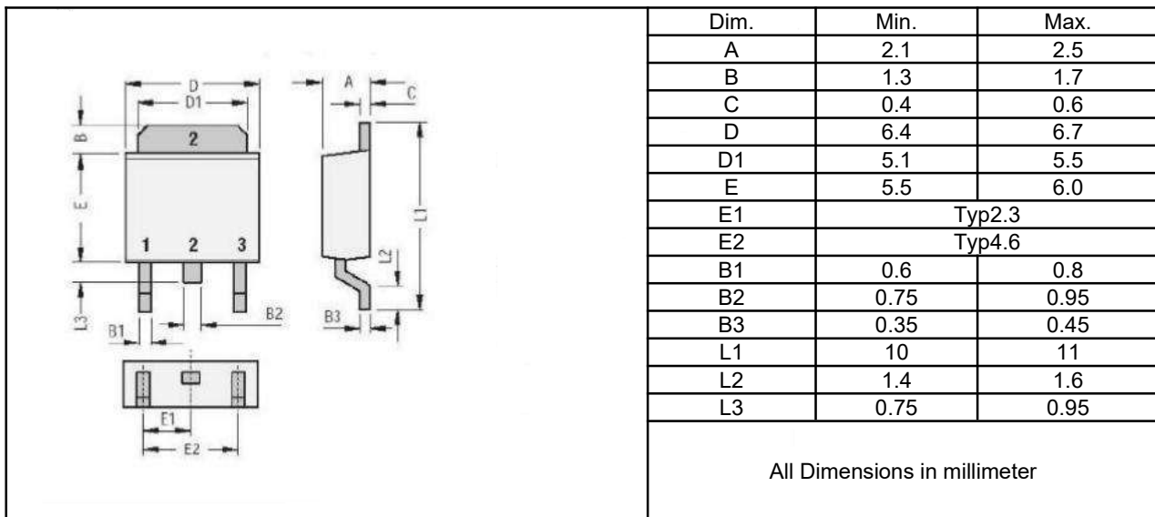
TO-252
