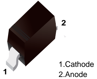
■ Simplified outline(SOD-323)
