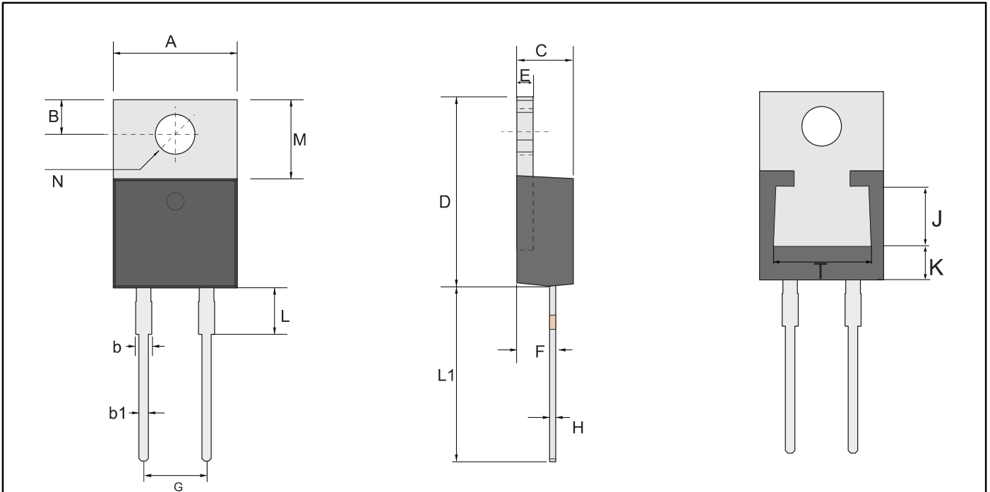
TO-220AC mechanical data
