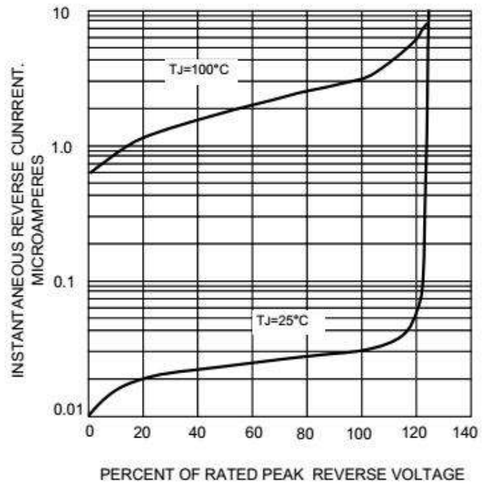
FIG.4-TYPICAL REVERSE CHARACTERISTICS
