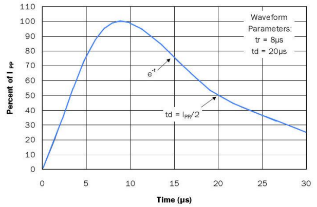
Figure 2- Pulse Waveform
